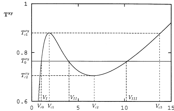
Fig. 3. Steady-state shear stress/shear rate curve for \eta_2 = 0.05 , We = 1 and \xi = 0.2 ; definition of various symbols.
