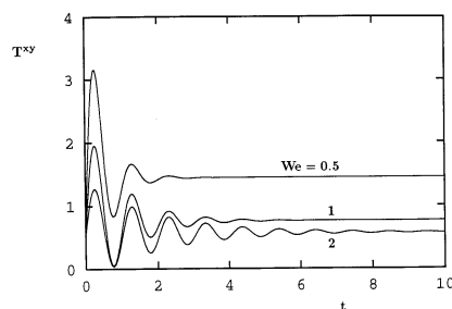
Fig. 7. Growth of T^{xy} during the inception of simple shear flow for zero Re , V = 10.2 and various values of We . It is assumed that a linear velocity profile is instantaneously attained. \eta_2 = 0.05 and \xi = 0.2 .
