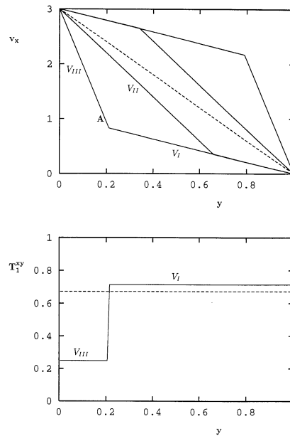
Fig. 4. (a) Steady-state solutions for v_x with one discontinuity point and corresponding to the same value of the shear stress. Solutions with a segment of slope V_{II} are unstable. (b) The component T_1^{xy} corresponding to profile A of Fig. 4a. The broken lines show the standard smooth solution. We = 1, \eta_2 = 0.05 , \zeta = 0.2 and V = 3 .
