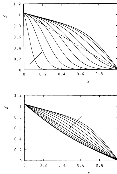
Fig. 9. Evolution of v_x during the inception of simple shear flow for V = 1.037 , Re = 1 , We = 1 , \eta_2 = 0.05 and \zeta = 0.2 : (a) times up to 1.05; (b) times from 1.05 to 2.05. The dashed line is the final steady-state.
