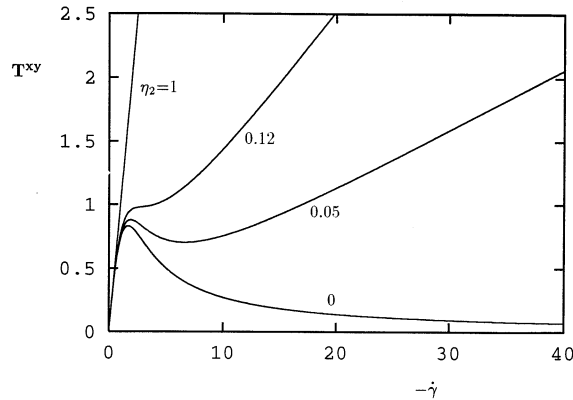
Fig. 2. Steady-state shear stress/shear rate curves for We = 1 , \xi = 0.2 and different values of \eta_2 . The curves for \eta_2 = 0.05 and 0 are calculated assuming that v_x is linear.
