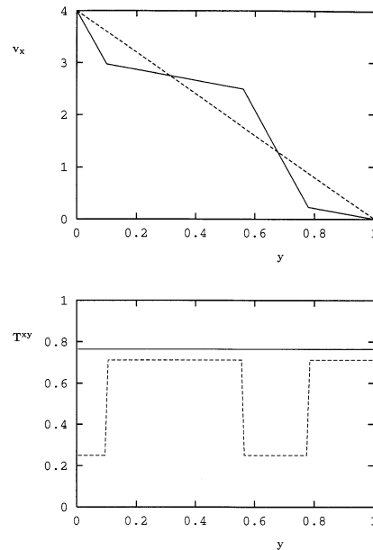
Fig. 14. One of the stable discontinuous steady-state solutions obtained for V=4 , Re=1 , We=1 , \eta_2=0.05 , \zeta=0.2 and V_0=3.9 : (a) velocity v_x ; the dashed line is the unstable smooth steady state; (b) shear stress T_i^{xy} ; the dashed line is T_1^{xy} .
