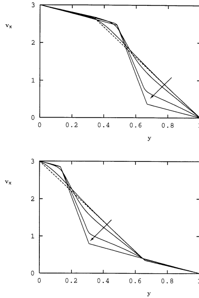
Fig. 17. Evolution of v_x after slightly perturbing the two unstable steady-state solutions of Fig. 4a ( V = 3 ). Dashed lines show the unstable solution. \text{Re} = 1 , \text{We} = 1 , \eta_2 = 0.05 and \zeta = 0.2 .
