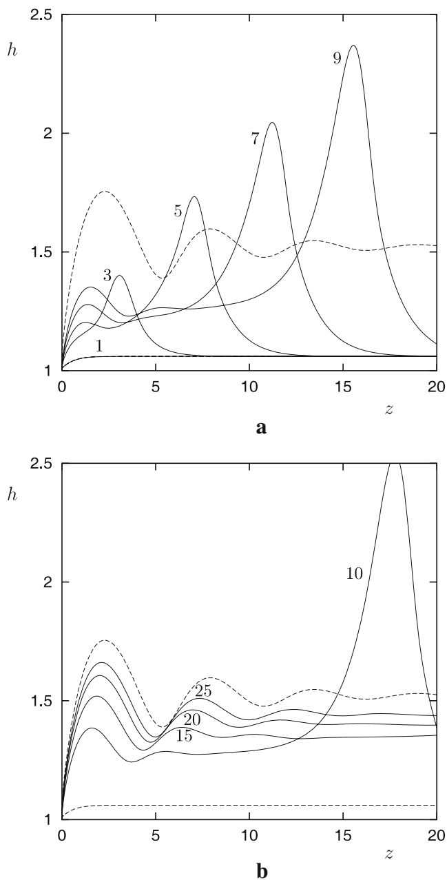
Fig. 22 Evolution of the free surface when perturbing the steady-state solution for B=0.06 and Re = 2.5 from Q_0 = 0.5 to Q = 1 : a t = 1, 3, 5, 7, and 9 ; b t = 10, 15, 20, 25 ; the dashed lines show the initial and the final steady state; axisymmetric flow with no slip at the wall, mesh 3 with L_1 = 5 and L_2 = 20
