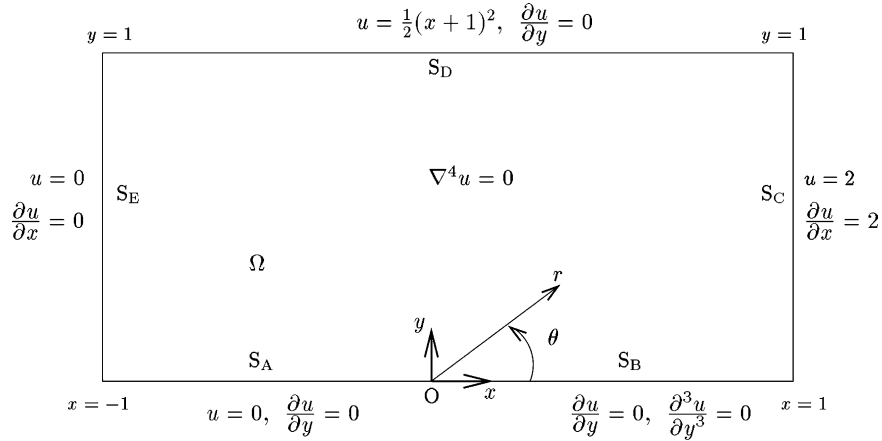
Fig. 2. The model fracture problem.
