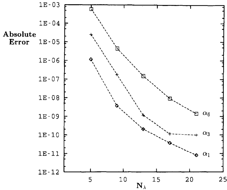
Fig. 4. Absolute errors as functions of N_x ; N_x=50 , singular function boundary integral method.
