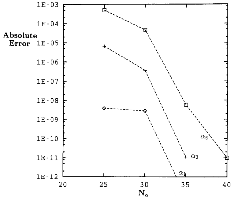
Fig. 5. Absolute errors as functions of N_\alpha ; N_\alpha=25 , singular function boundary integral method.
