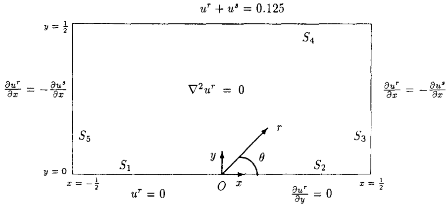
Fig. 2. The modified cracked-beam problem.
