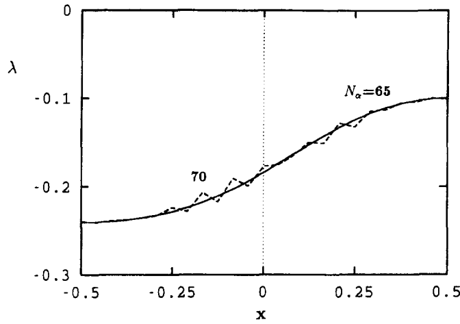
Fig. 3. Calculated Lagrange multipliers for N_\alpha=65 and 70; N_i=25 , singular function boundary integral method.
