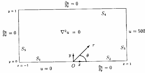
Figure 1. The Motz problem
