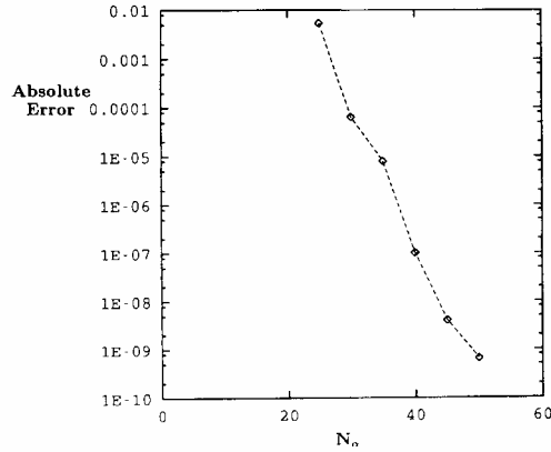
Figure 4. Absolute error of \alpha_{15} , as a function of N_u ( N_\lambda = 25 )
