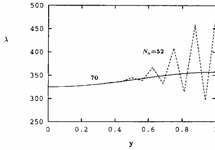
Figure 2. Calculated Lagrange multipliers for N_o = 52 and 70 ( N_\lambda = 17 )
