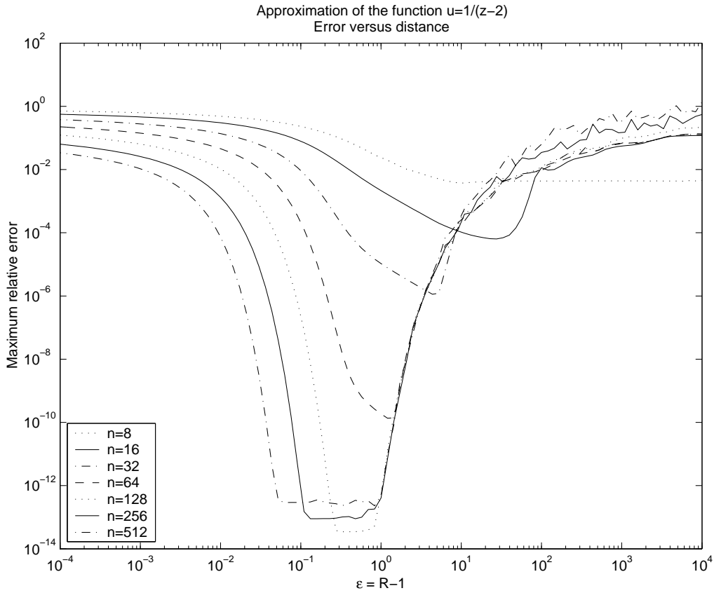
FIGURE 1. Log of maximum relative error versus log \varepsilon in Example 1.
